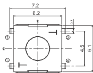
Figure 2 – 222CJ, Surface Mount J-Bend
